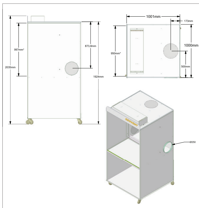
Spray booth for smaller items
