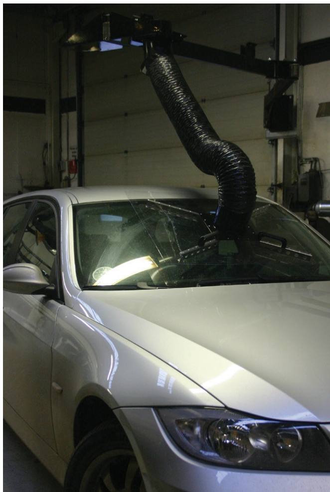
Extraction hood for windscreen gluing in use.
